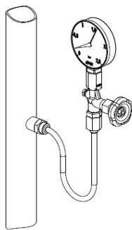
Vertical pipes
