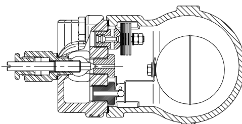
FLT17LC-FLT4I DN15-20
